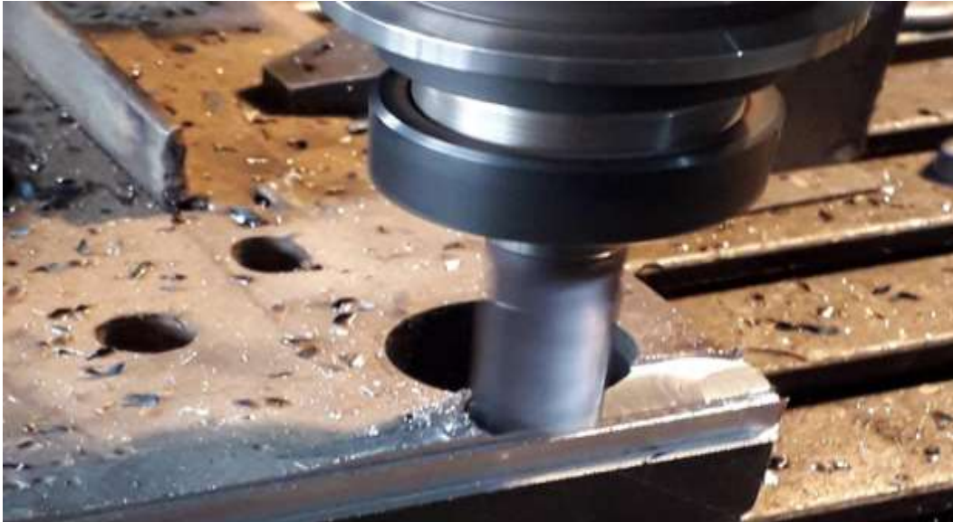
Figure 4. The process of processing with the help of finger milling
