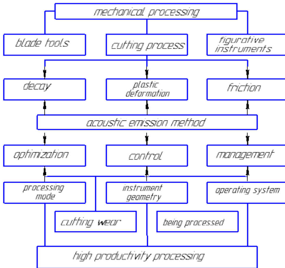
Figure 4. As shown in the diagram , mechanical processing using acoustic emission ( VAS ). From the VAS method structural diagram of use in the processing of changes in cutting conditions. Because VAS is produced by basic physical processing processes, experiments have shown that any change in their energy capacity leads to a change in acoustic radiation parameters. The main treatment factors diagnosed with this method are: chip formation and collapse. The onset of chip crushing is usually accompanied by a characteristic increase in signal VAS, which can be used to control vibration sharpening, drilling, especially the recording process; sharpening geometry and brand of tool materials, as well as the effect of wear-resistant coating; rigidity of process system elements; the effect of physical and mechanical properties of materials on processing; the type of technological environment used, its concentration; surface quality and the presence of a recyclable structure material; knife and abrasive tool wear; surface depth and pre-processing methods. Thus, the VAS method allows the identification of all important processing properties and, especially valuable ones, to determine their interactions. This predetermines the possibility of using VAS signals to control the intersection. A block diagram of the application of the VAS method in machining operations is shown.
